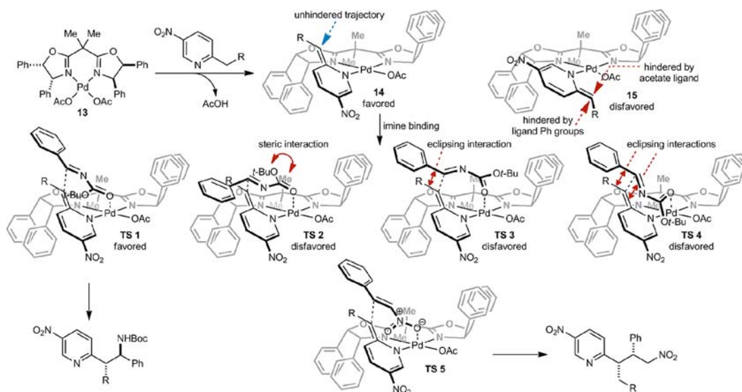
Figure 2. Stereochemical model.
